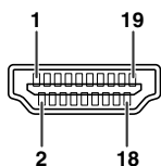
HDMI Terminal
